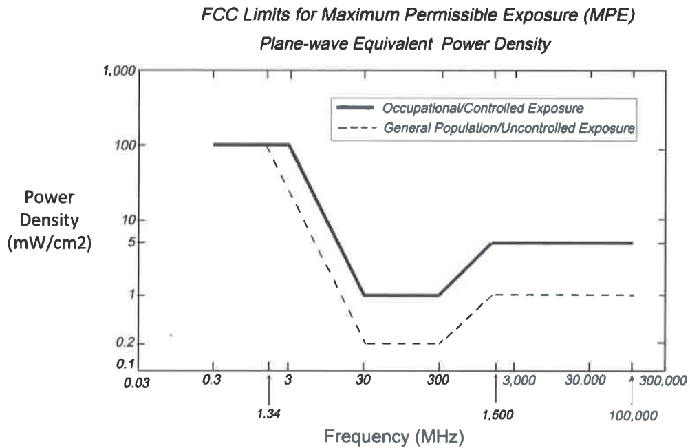
Figure 3 FCC Human Wireless Radiation Exposure Limits
